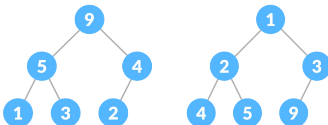
Max Heap
